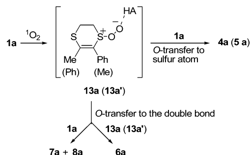
SCHEME 7
