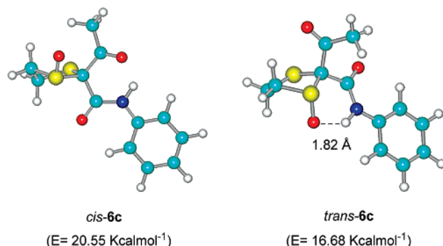
FIGURE 3. Theoretical calculations.
