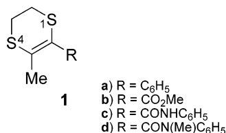
FIGURE 1. 2,3-Disubstituted dithiins.
